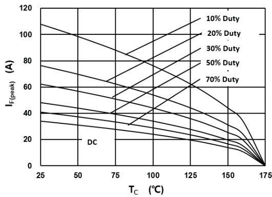
Fig 3: Current Derating
