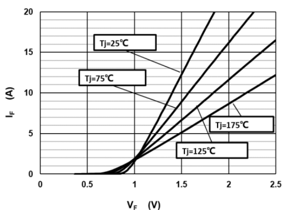
Fig 1: Forward Characteristics
