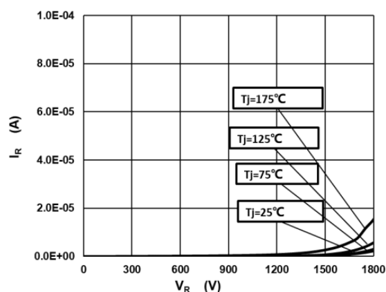
Fig 2: Reverse Characteristics
