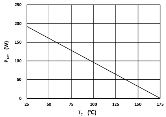
Fig 4: Power Derating
